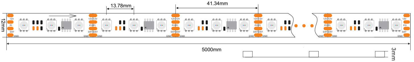
Dimensional Drawing of DC12V 72LED/M DMX512 LED Strip
