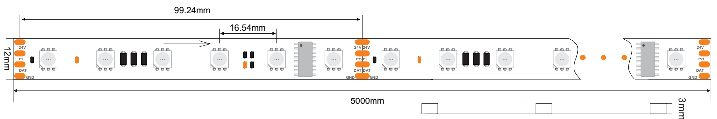
Dimensional Drawing of DC24V 60LED/M DMX512 LED Strip
