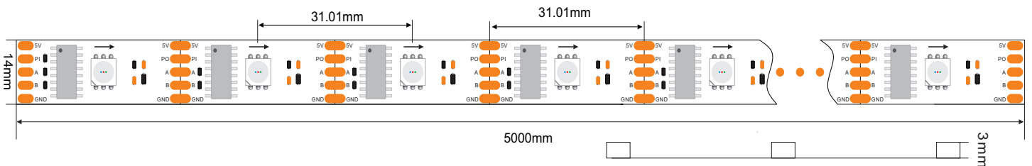
Dimensional Drawing of DC5V 32LED/M DMX512 LED Strip
