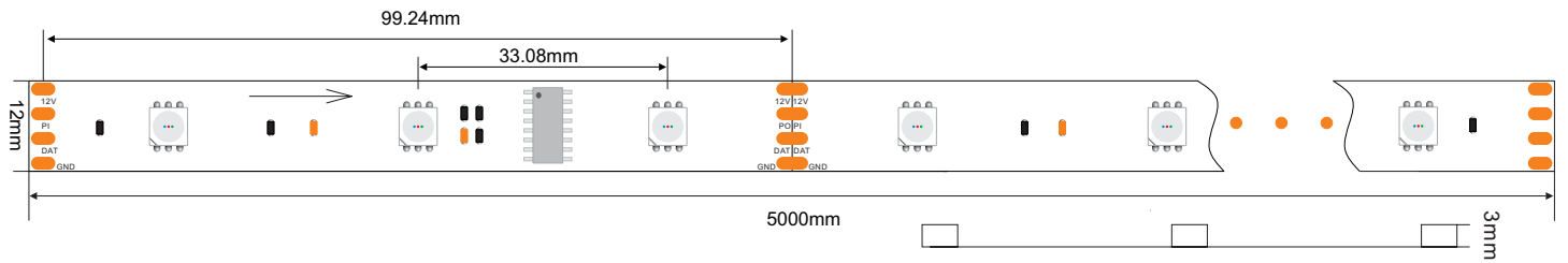
Dimensional Drawing of DC12V 30LED/M DMX512 LED Strip
