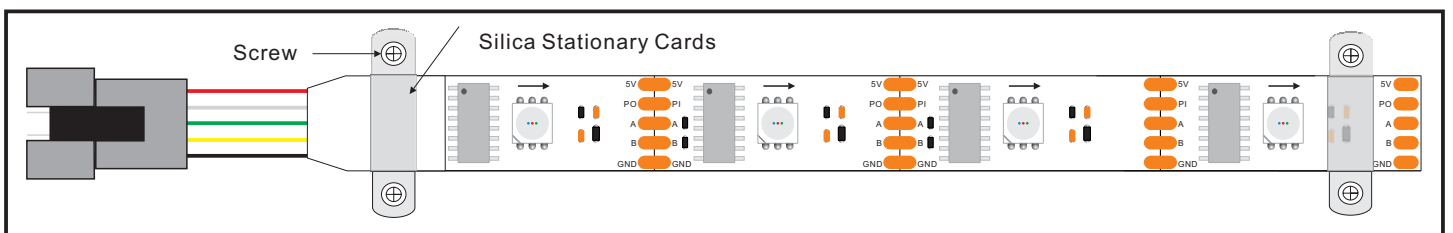
Put the led strip on install place , use screw to fixed , each meter need to use 2 silicone snap
